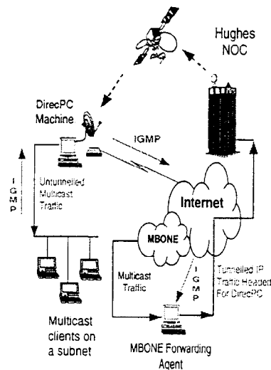
Figure 5: Tunneled Multicast with IGMP Forwarding
